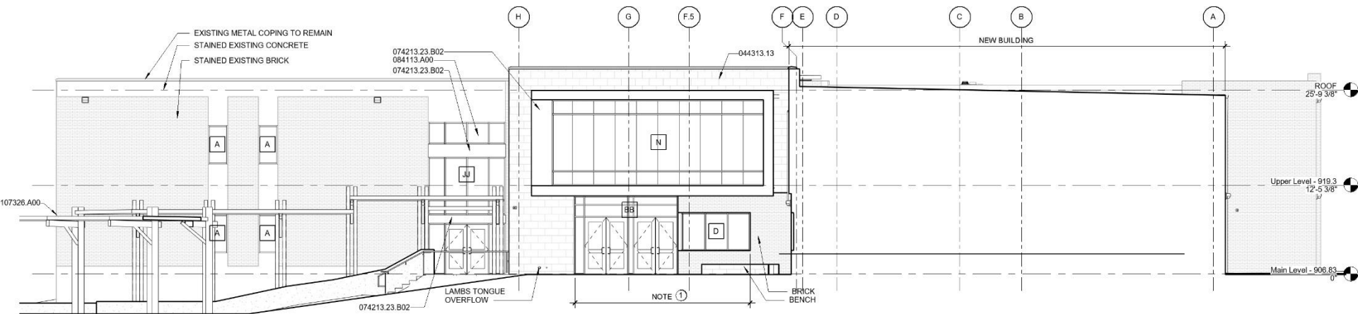
Building Elevation - North
